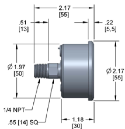
20-911 1/4" NPT
