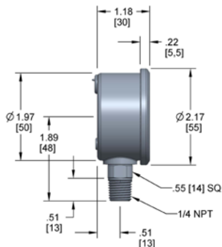
20-911 1/4" NPT
