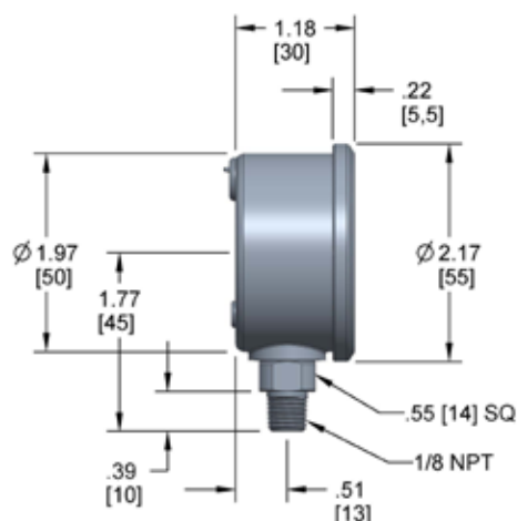
20-911 1/8" NPT
