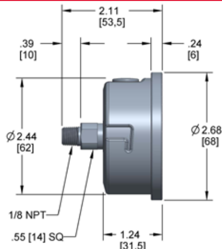
25-911 1/8" NPT
