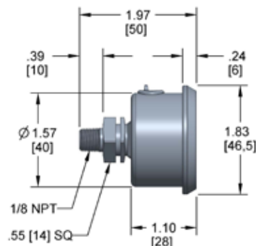
15-911 1/8" NPT
