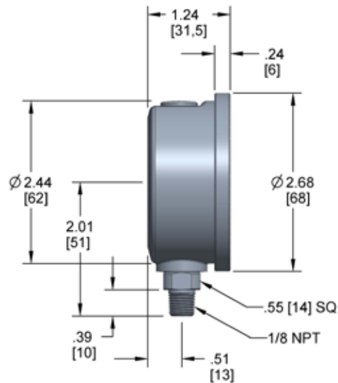
25-910 1/8" NPT
