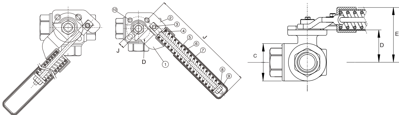
CLOSE CONDITION
