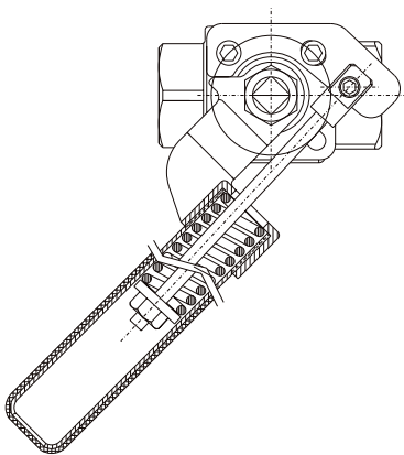
OPEN CONDITION
